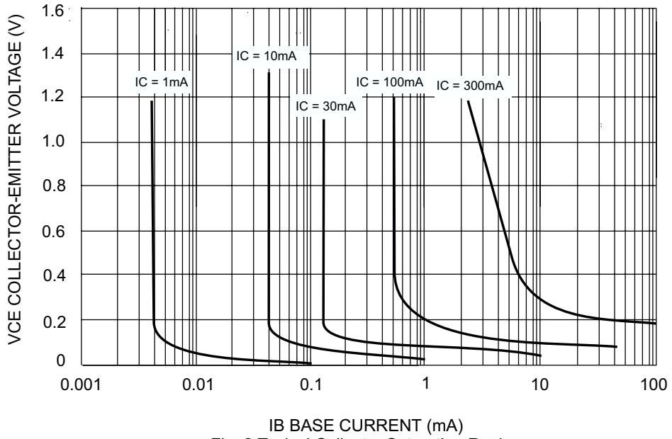
Fig. 2 Typical Collector Saturation Region
